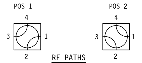
* PATENTED STD. ELECTRICAL CKT. Shown in Position 1 ONE FORM C
