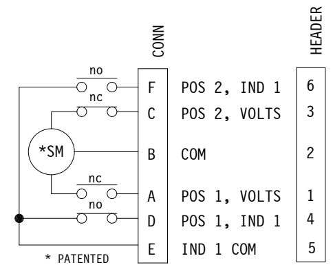
STD. ELECTRICAL CKT. Shown in Position 1 ONE FORM C
