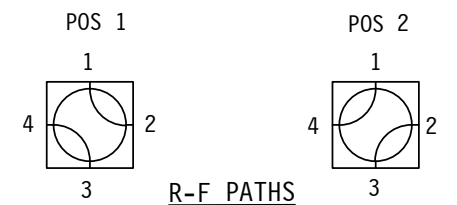
STD. ELECTRICAL CKT. Shown in Position 1 ONE FORM C
