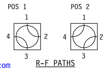
* PATENTED STD. ELECTRICAL CKT. Shown in Position 1 ONE FORM C
