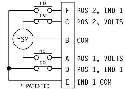
* PATENTED STD. ELECTRICAL CKT. Shown in Position 1 ONE FORM C
